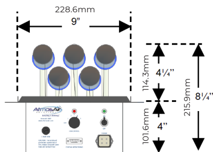
Duct Cut-Out
